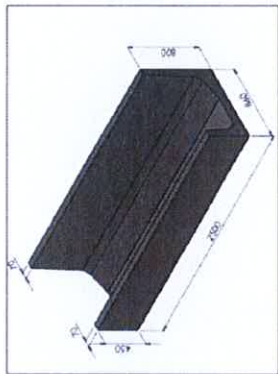
PRE-CAST FEED TROUGHS
