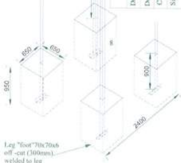
FOUNDATION: TANKSTAND
