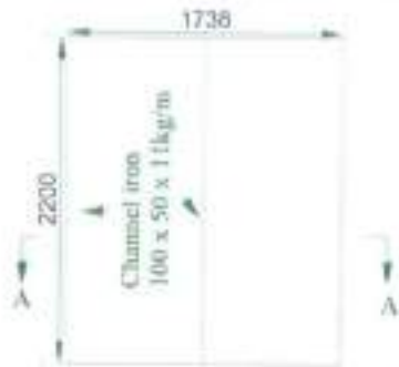
TOP VIEW : Carrier and support beams
