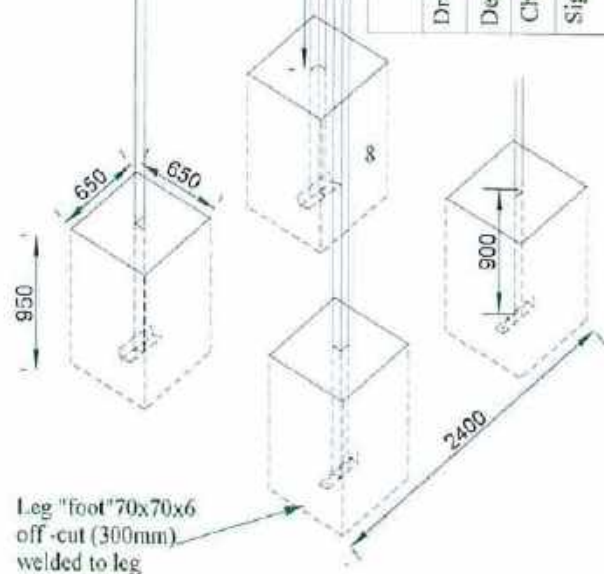
FOUNDATION: TANKSTAND
