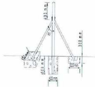
Corner post - detail
