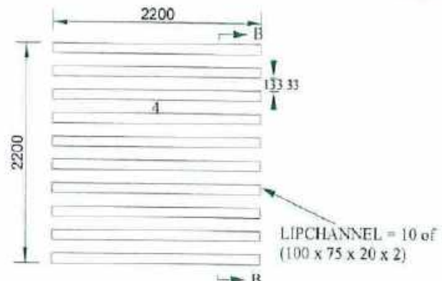
TOP VIEW : Platform
