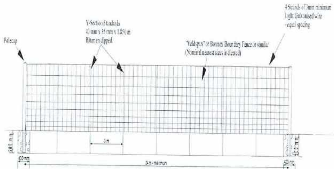
"Veldspan" - Detail
