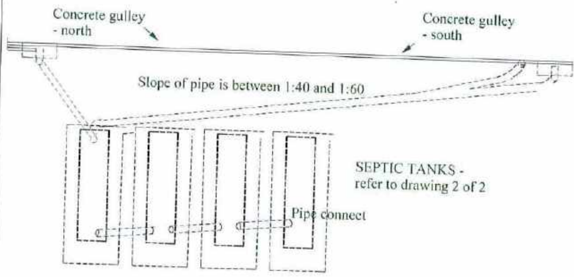
SECTION VIEW - Not to scale
