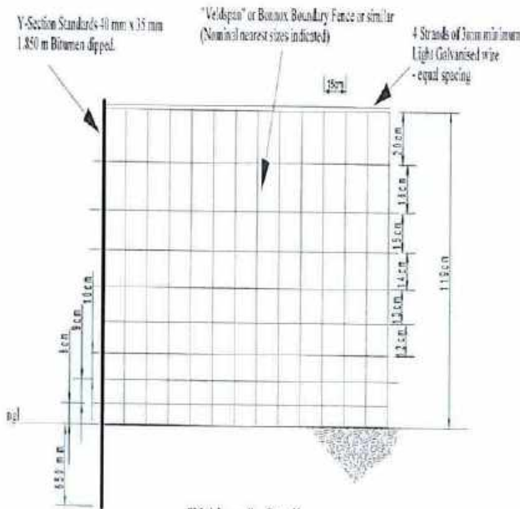
"Veldspan" - Detail
